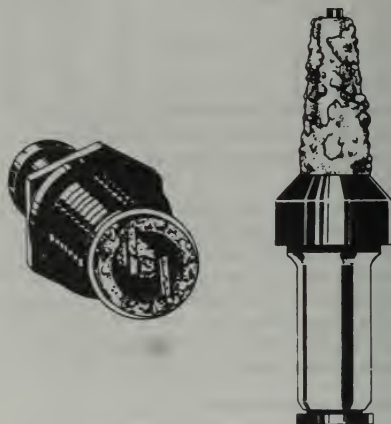
FIGURE 4-53. Lead-fouled spark plug.
